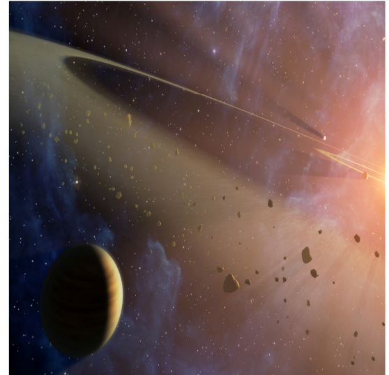
This artist's illustration shows an asteroid belt full of rocky bodies of different sizes and compositions that orbit the Sun. Some of these are near-Earth objects (NEOs) that travel within 1.3 AU of Earth. Credit: NASA/JPL-Caltech
