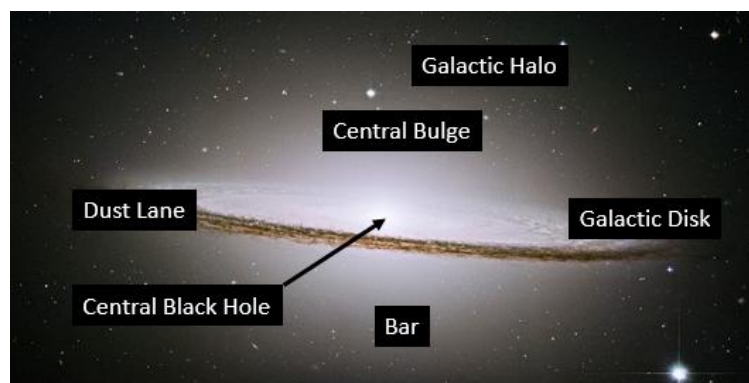
Figure 390: Parts of a Spiral Galaxy
