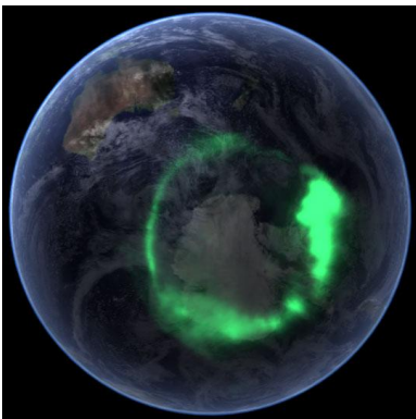
Figure 125: South Pole Auroral Oval
