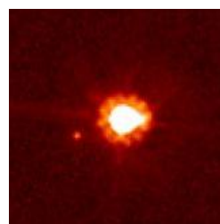
Figure 243: Eris and Dysnomia
