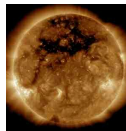
Figure 293: Coronal Hole
