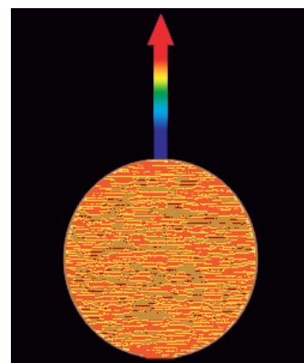
Figure 352: Gravitational Redshift
