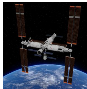
Figure 167e: Tiangong Space Station
