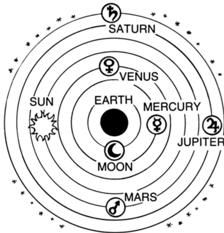
Figure 48: Ptolemy's Model of the Universe - Geocentric
