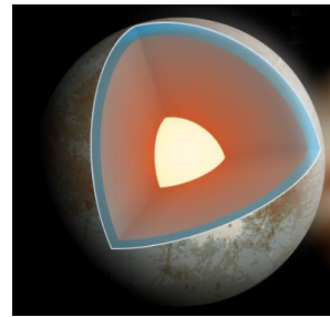
Figure 194: Europa's Interior
