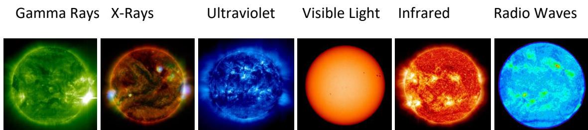
Figure 278: The Sun at different Frequencies
