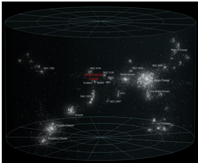
Figure 6: Virgo Supercluster
