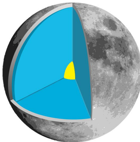
Figure 128: The Moon's Internal Structure
