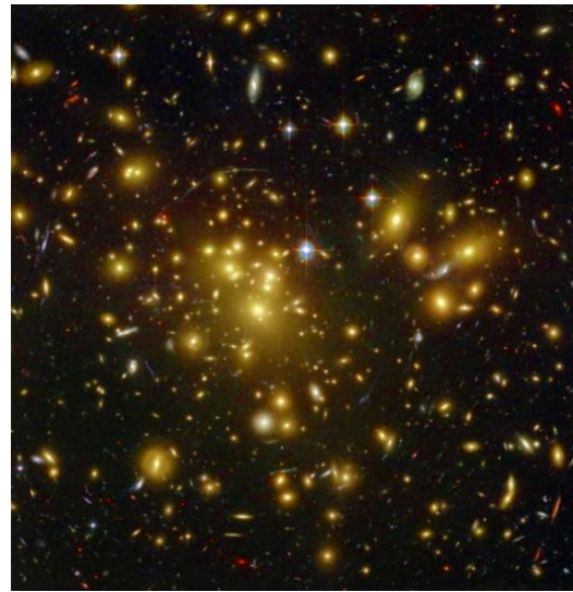
Figure 353: Gravitational Lensing
