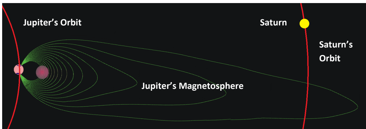
Figure 185: Jupiter's Magnetosphere
