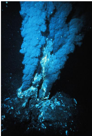
Figure 117: Mid-Atlantic Ridge
