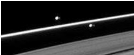
Figure 219: Shepherd Moons
