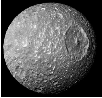
Figure 214: Mimas
