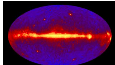
Figure 117: Gamma Ray All Sky Survey (EGRET)
