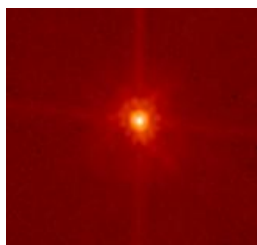
Figure 244: Makemake
