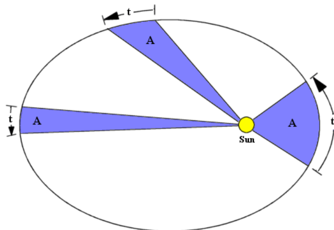
Figure 56: Kepler's 2nd Law
