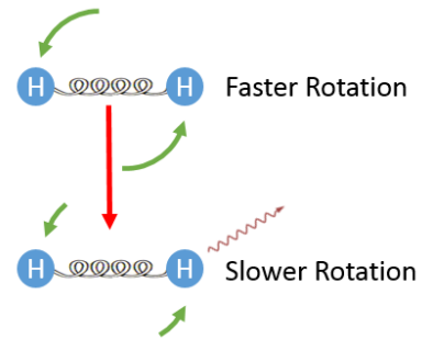
Figure 137: Molecular Rotation
