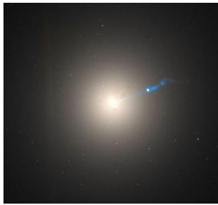
Figure 374: Type E0 Elliptical Galaxy
