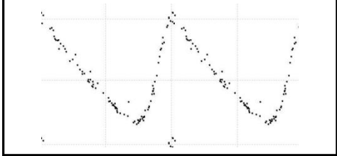
Figure 146: Cepheid Light Curve
