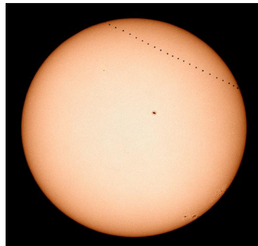
Figure 139: Mercury Transit - 2003
