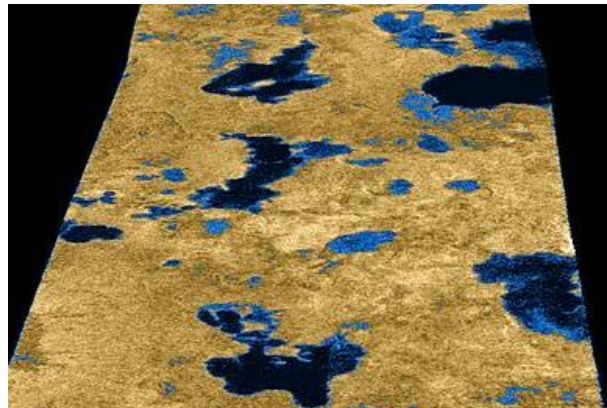
Figure 211: Titan's Methane Lakes
