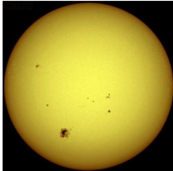
Figure 2: The Sun – 870,000 miles diameter
