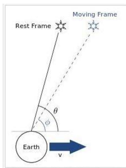
Figure 493: Effect of Earth's Velocity
