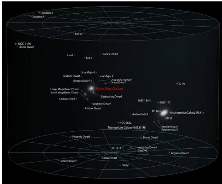
Figure 7: The Local Galaxy Group
