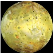
Figure 188: Io
