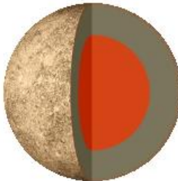
Figure 133: Mercury's Internal Structure
