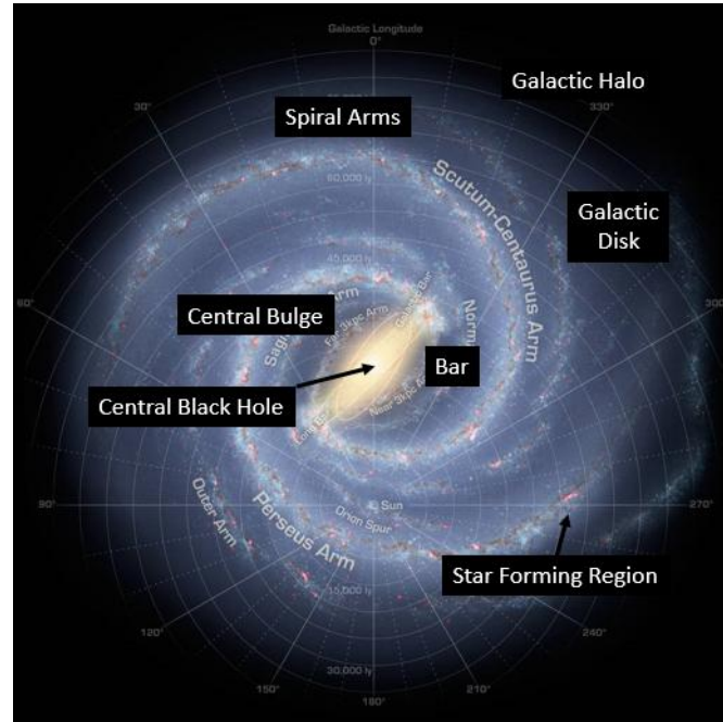
Figure 365: Parts of a Barred Spiral Galaxy
