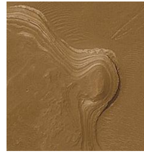
Figure 172: Erosion by Standing Water
