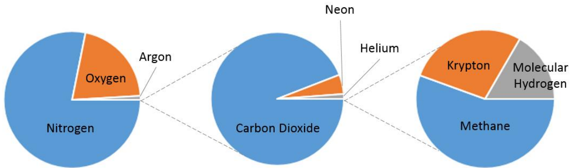
Figure 109: Earth's Atmosphere Components
