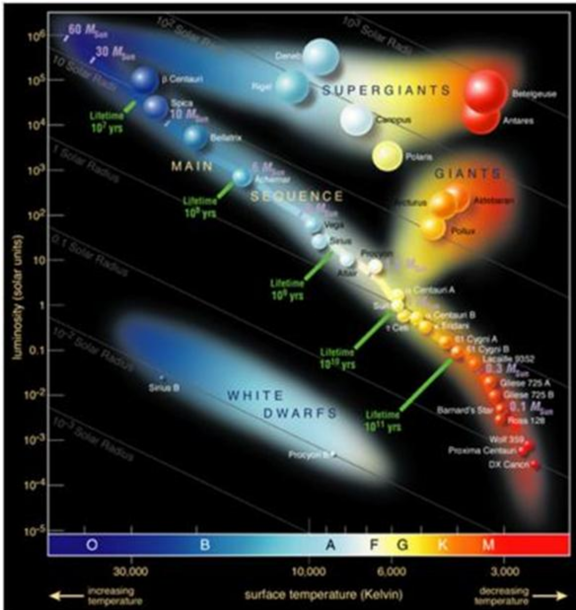
Figure 503: HR Diagram
