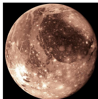
Figure 448: Ganymede
