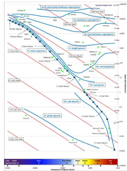
Figure 144: The HR Diagram
