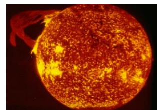
Figure 290: Solar Flares
