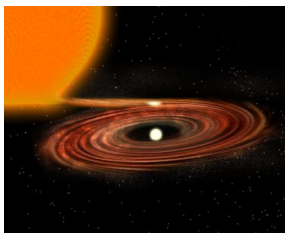
Figure 360: Accretion Disk
