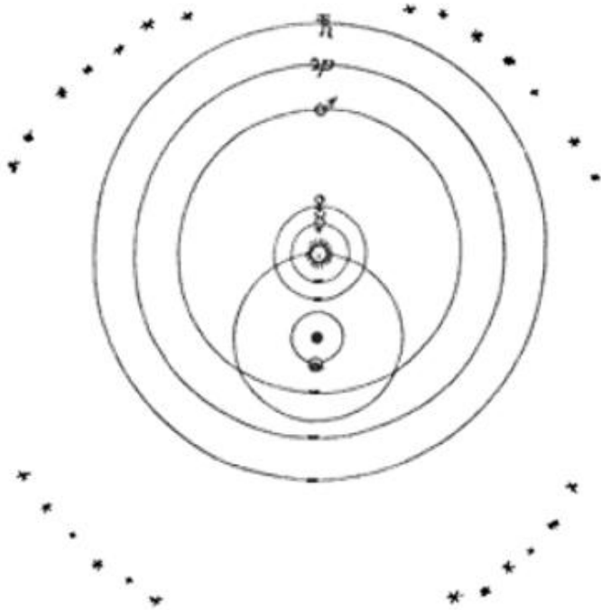
Figure 54: Brahe's Model of the Universe
