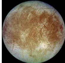
Figure 189: Europa
