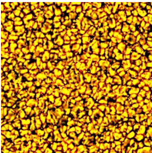
Figure 285: Granulation
