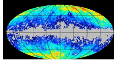
Figure 111: Ultraviolet All Sky Survey (GALEX)
