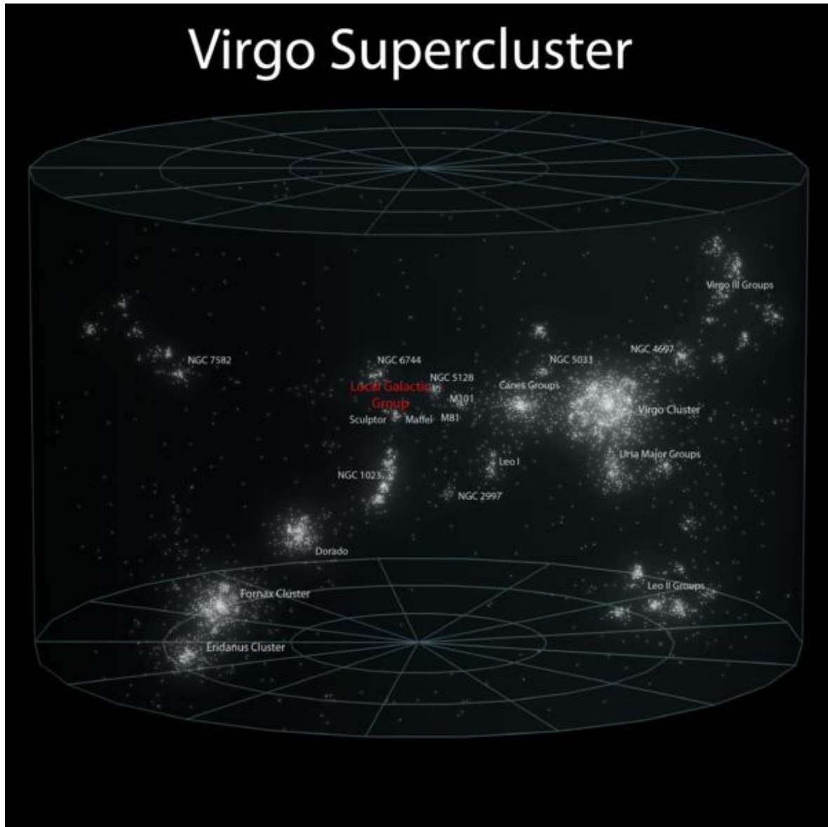
Figure 383: The Local Galaxy Supercluster
