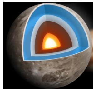
Figure 195: Ganymede's Interior
