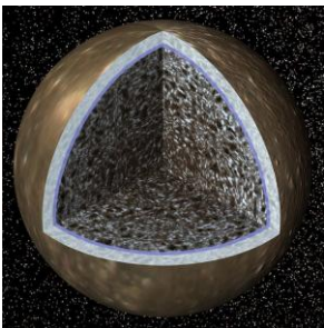
Figure 196: Callisto's Interior
