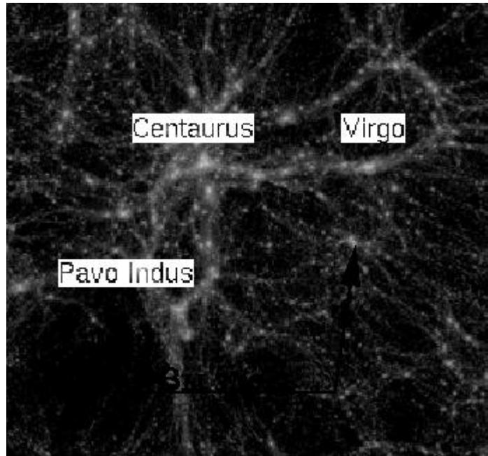
Figure 8: The Local Supercluster
