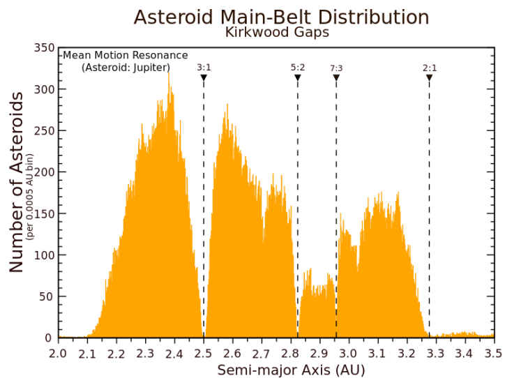
Figure 250: Kirkwood Gaps
