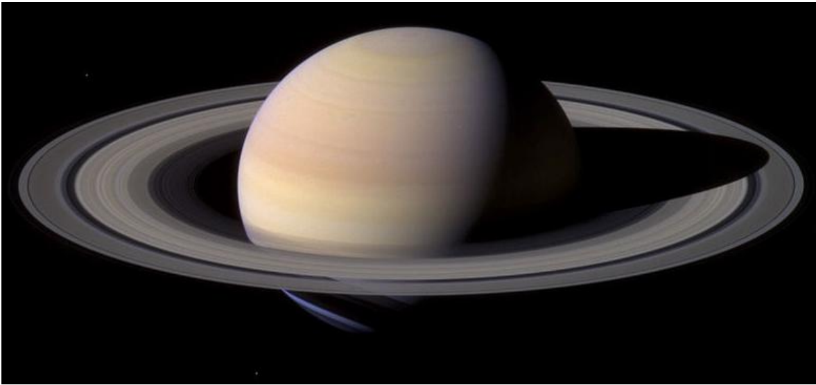
Figure 216: Saturn's Rings
