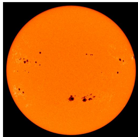
Figure 275: The Sun
