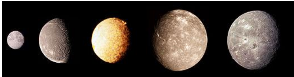
Figure 228: Uranus' Moons
