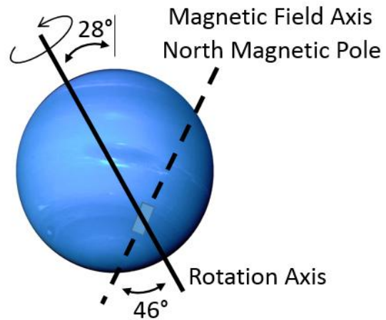
Figure 235: Neptune's Magnetic Field
