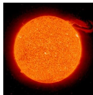
Figure 291: Solar Prominence
