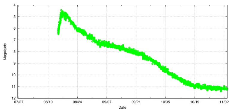
Figure 359: Nova Delphinus 2013
