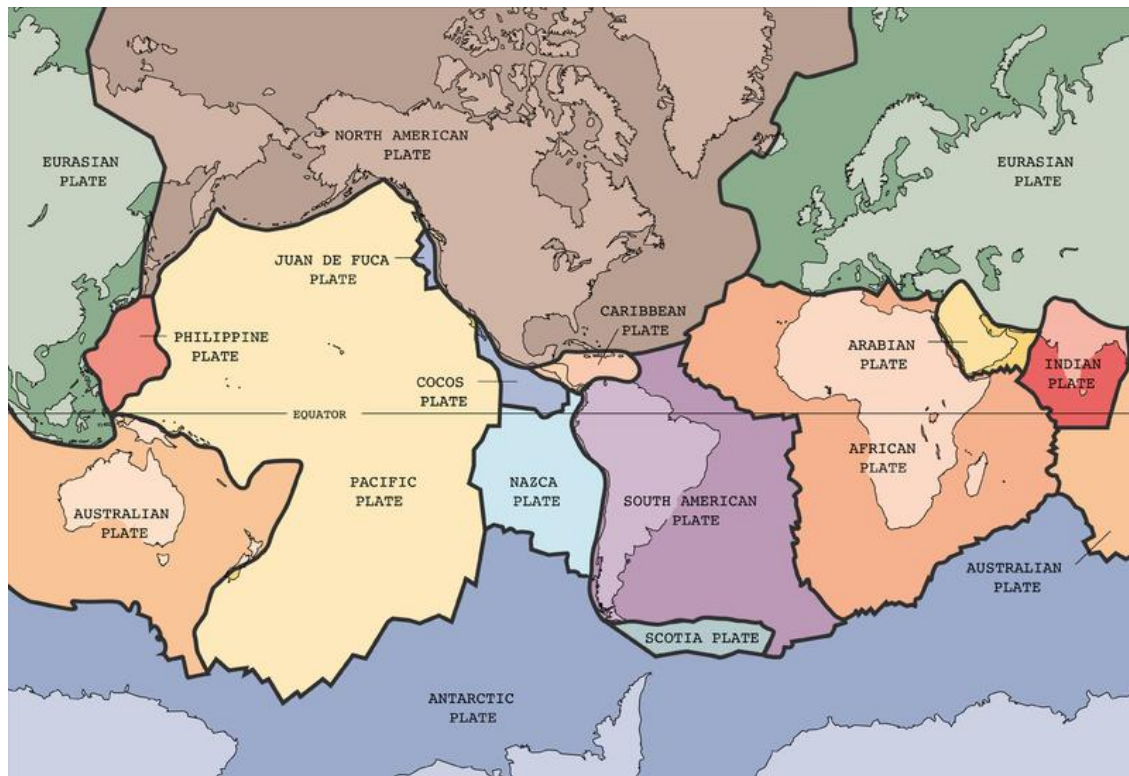
Figure 113: Tectonic Plates
