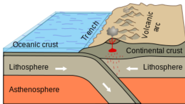
Figure 119: Subduction
