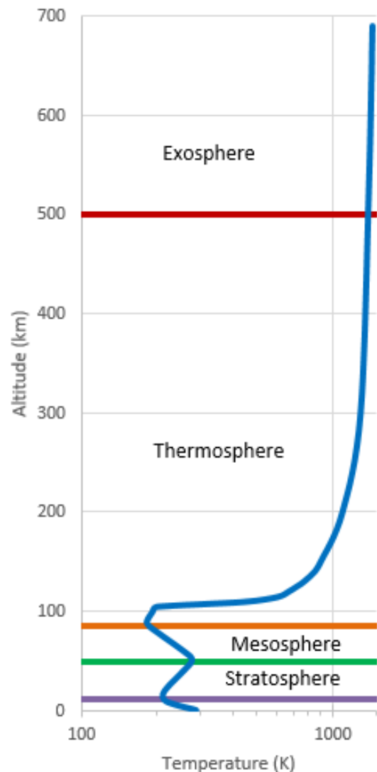
Figure 108: Earth's Atmosphere Profile
