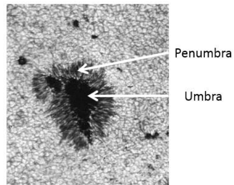
Figure 286: Sunspots
