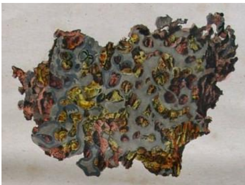
Figure 267: Inside a Stoney-Iron Meteorite
