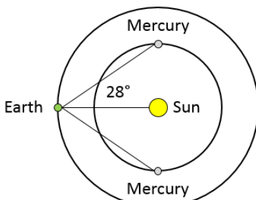
Figure 140: Mercury at Greatest Elongation
