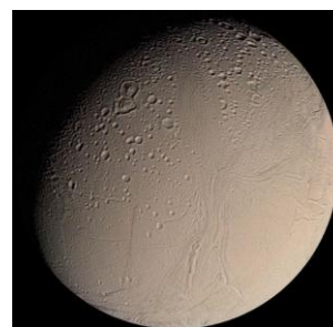
Figure 450: Enceladus
