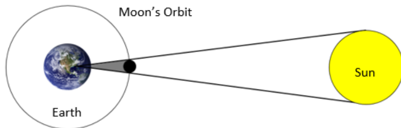
Figure 31: Solar Eclipses
