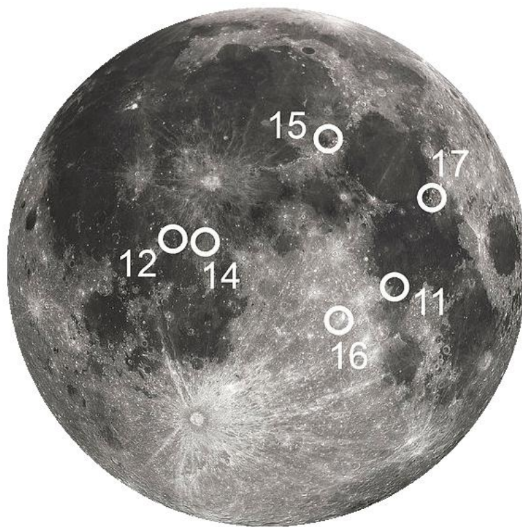
Figure 131: The Apollo Landing Sites
