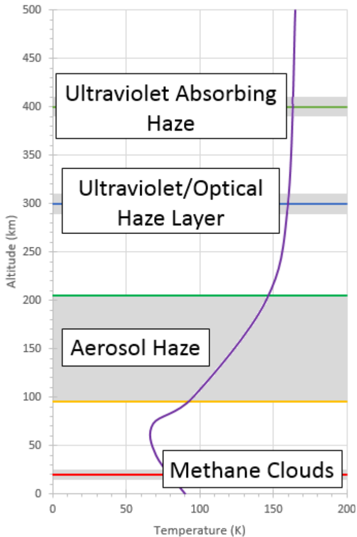
Figure 213: Titan's Atmospheric Profile
