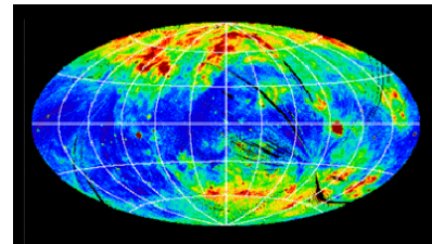
Figure 115: X-Ray All Sky Survey (ROSAT)
