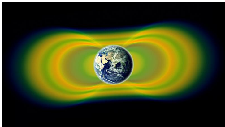
Figure 122: The Van Allen Radiation Belts
