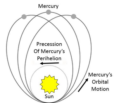
Figure 356: Mercury's Orbital Motion
