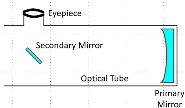
Figure 91: Parts of a Newtonian Telescope
