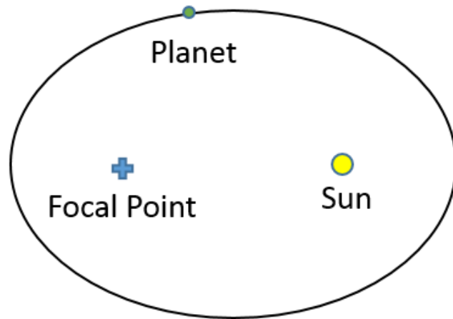
Figure 55: Kepler's 1st Law
