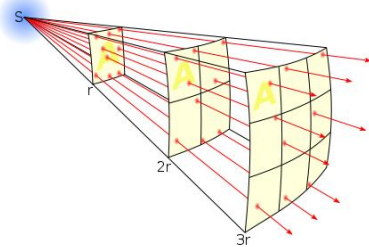
Figure 298: Inverse-Square Law
