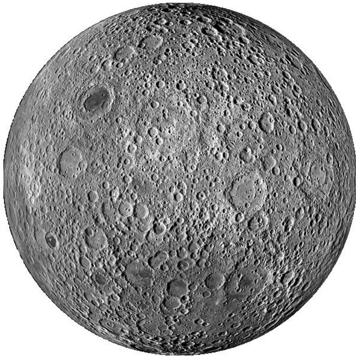
Figure 129: The Far Side of the Moon
