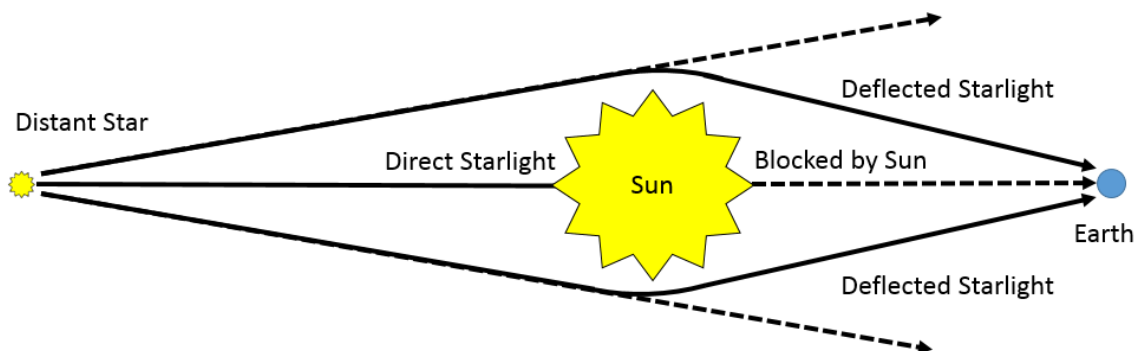
Figure 354: Starlight Deflected by the Sun
