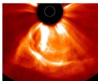
Figure 292: Coronal Mass Ejection
