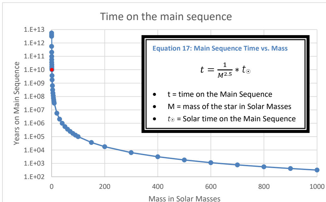
Figure 313: Main Sequence Time vs. Mass
