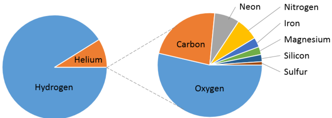
Figure 276: The Sun's Atmosphere
