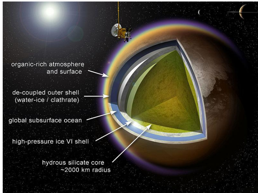
Figure 210: Structure of Titan
