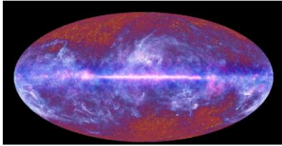
Figure 110: Radio All Sky Survey (PLANCK)
