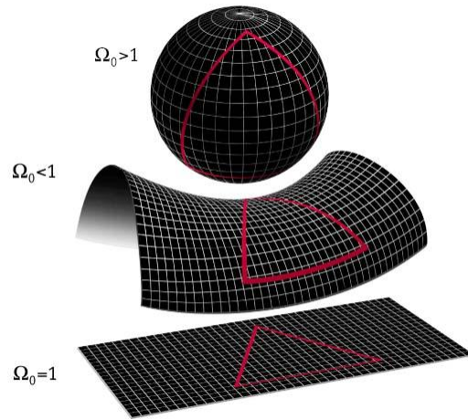
Figure 424: An Open, Closed, or Flat Universe
