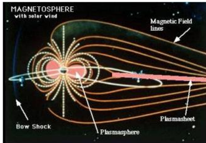
Figure 121: The Earth's Magnetosphere
