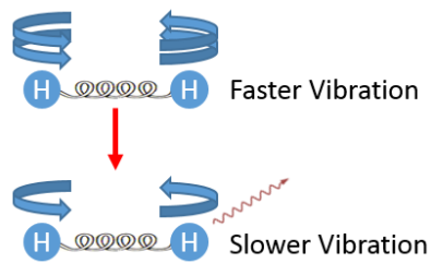
Figure 138: Molecular Vibration
