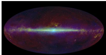
Figure 112: Infrared All Sky Survey (WISE)
