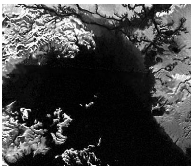
Figure 449: Titan's Surface
