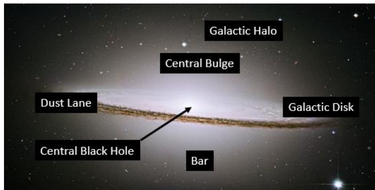
Figure 366: Parts of a Spiral Galaxy
