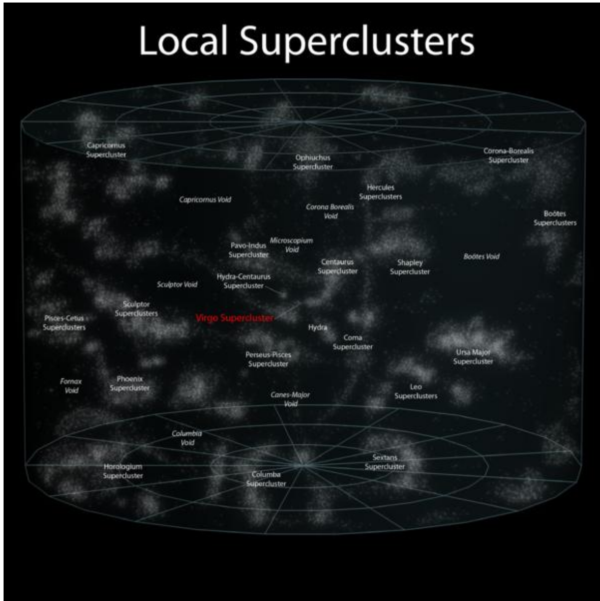
Figure 384: The Local Superclusters of Galaxies
