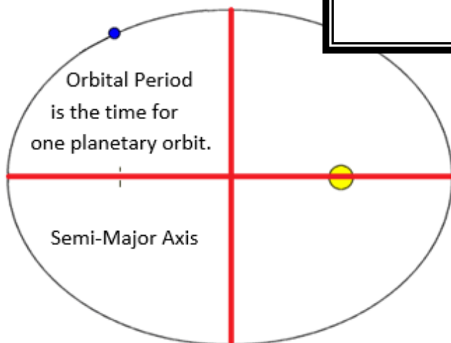
Figure 57: Kepler's 3rd Law
