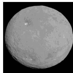
Figure 242: Ceres
