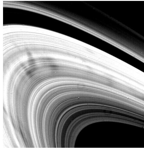
Figure 218: Spokes in the Rings
