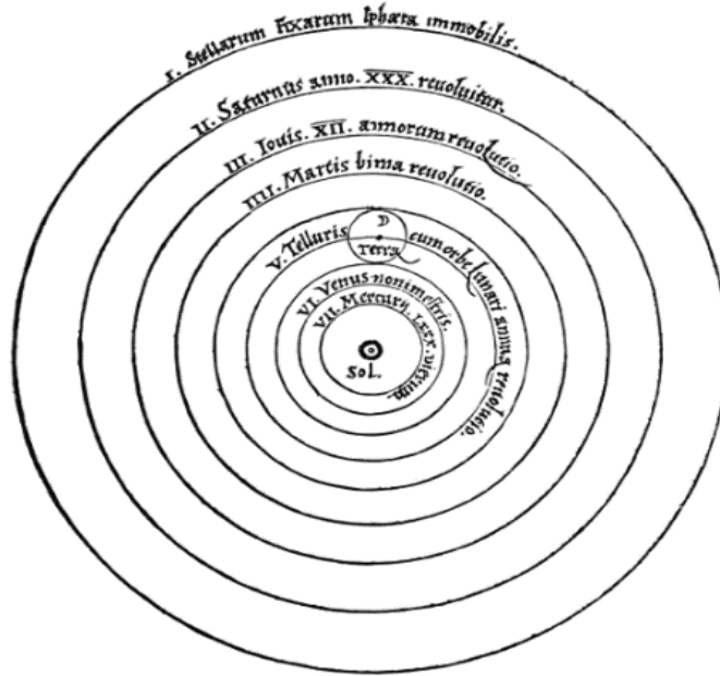
Figure 52: Kepler's Model of the Solar System - Heliocentric
