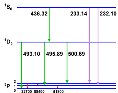
Figure 334: Forbidden Lines
