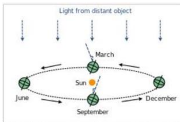
Figure 492: Stellar Aberration
