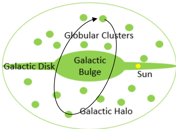
Figure 395: Globular Cluster Location
