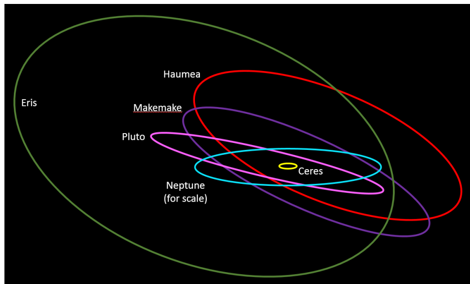
Figure 247: Dwarf Planet Orbits
