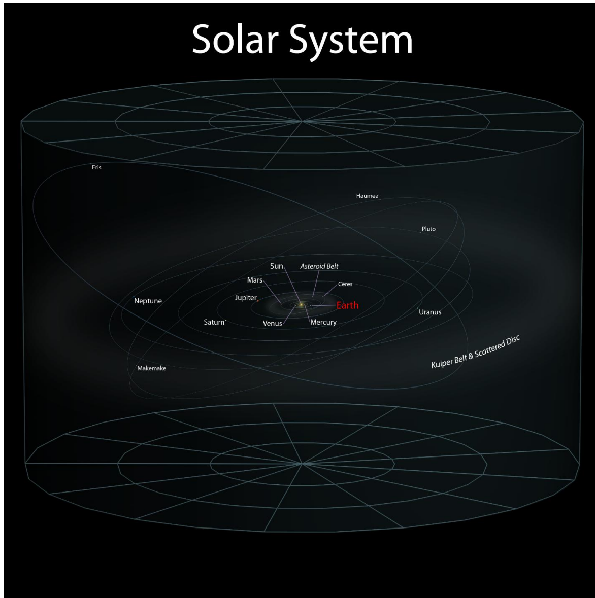
Figure 248: Solar System Layout
