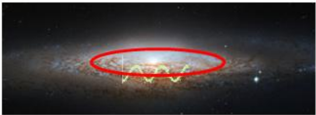
Figure 23: The Sun's Orbital Oscillations
