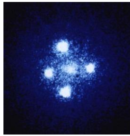
Figure 355: Einstein Cross
