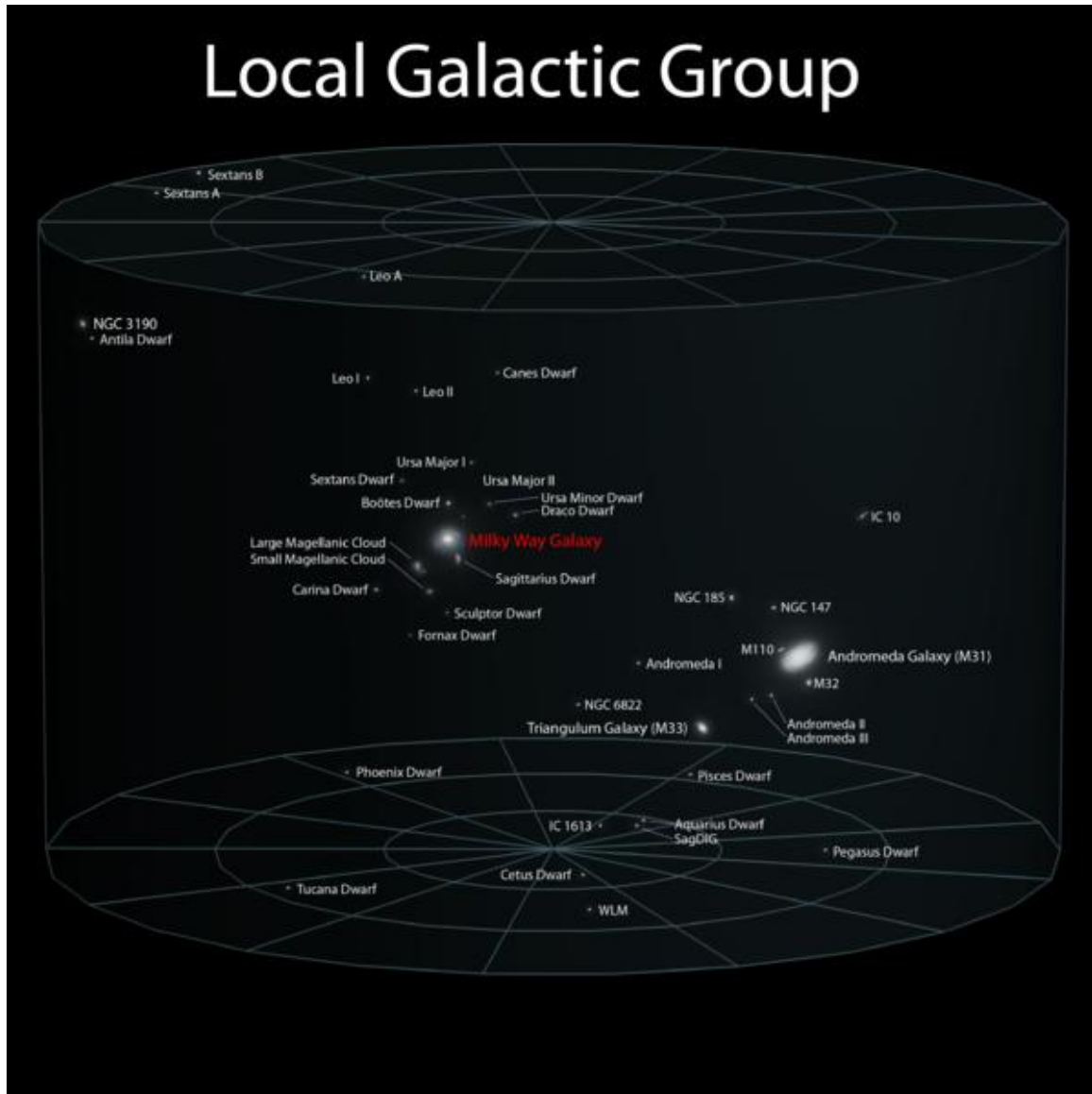
Figure 382: The Local Galaxy Cluster
