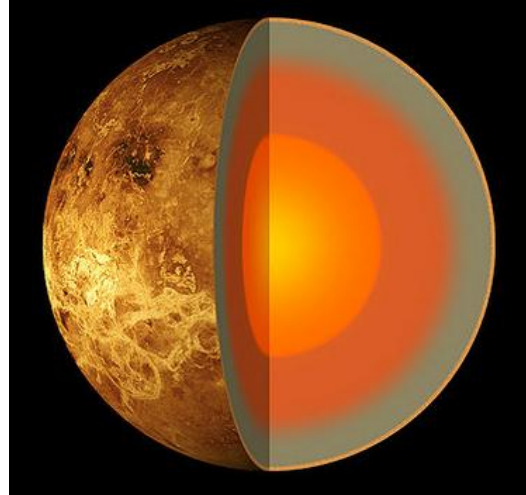
Figure 141: Venus' Internal Structure
