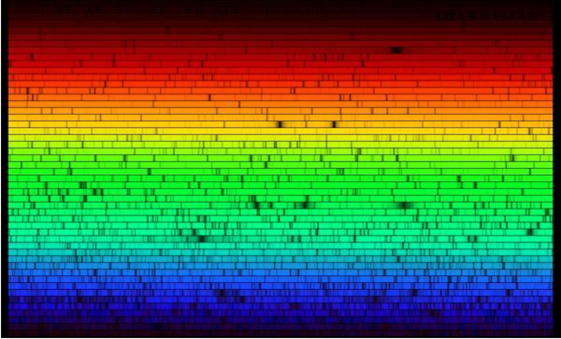
Figure 277: The Sun's Spectrum
