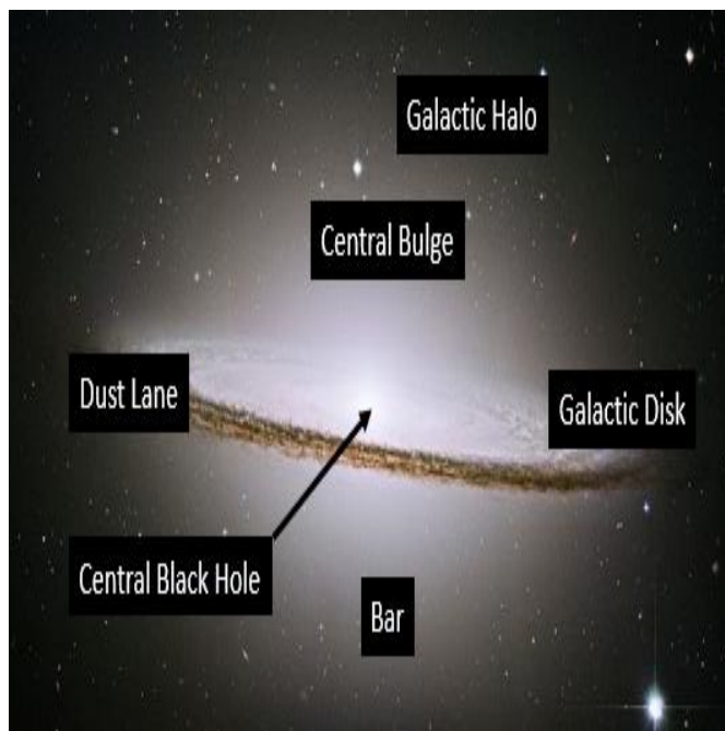
Figure 389: Parts of a Barred Spiral Galaxy
