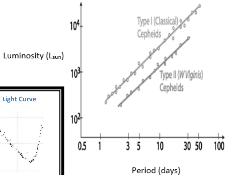
Figure 145: Luminosity of Cepheid Variable Stars
