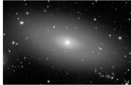
Figure 367: Type S0 Galaxy
