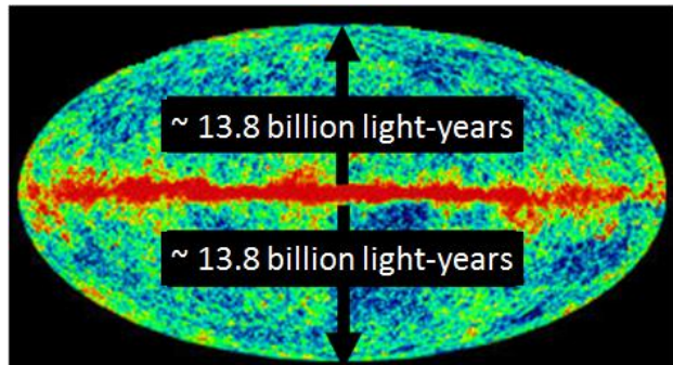
Figure 431: The Horizon
