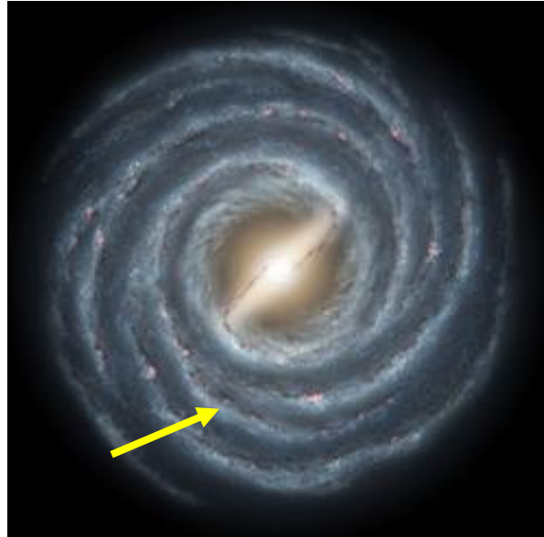
Figure 4: The Milky Way Galaxy
