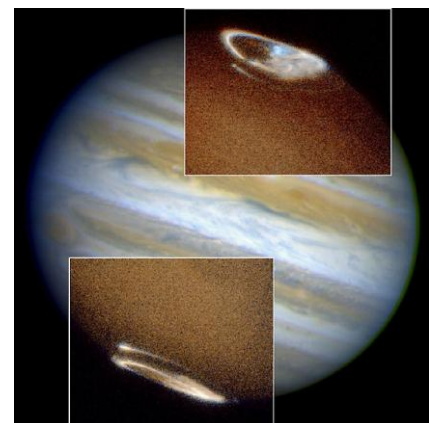
Figure 186: Jupiter's Aurorae
