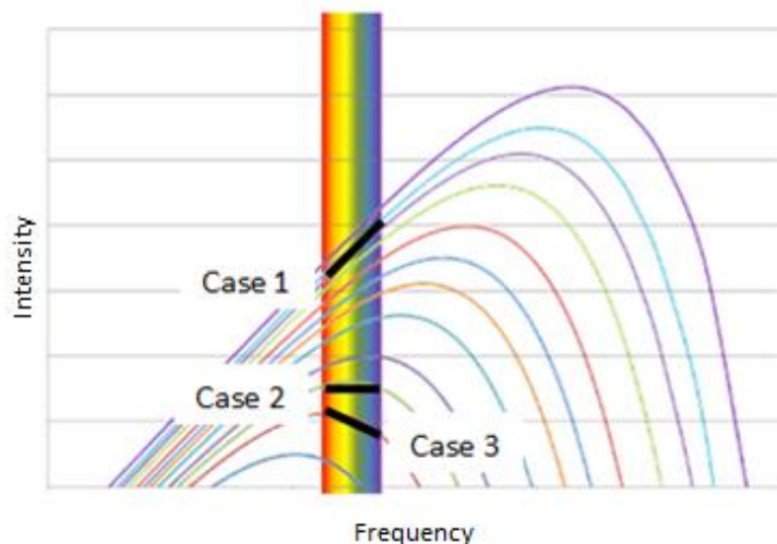
Figure 299: Filtered Intensities
