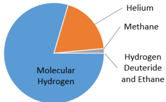
Figure 234: Neptune's Atmospheric Composition
