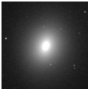
Figure 376: Type E2 Elliptical Galaxy
